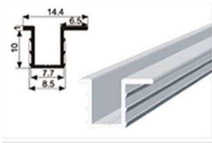
U PROFILE (1786)
